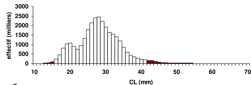
strate vase 75% (VS)
